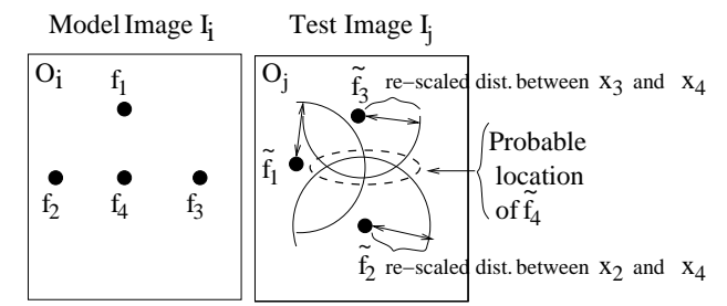
Figure 1. Example of position prediction. Given the features from the model \{\mathbf{f}_l\} and their correspondences \{\tilde{\mathbf{f}}_l\} , for l = \{1, 2, 3\} , we want to estimate the position of \tilde{\mathbf{f}}_4 . Its probable location (represented by a dotted ellipsoid) is based on a Gaussian distribution computed using the position of the correspondences in the test and model images and the pairwise variances \sigma_D^2(\mathbf{f}_l, \mathbf{f}_o) estimated in the learning stage.
