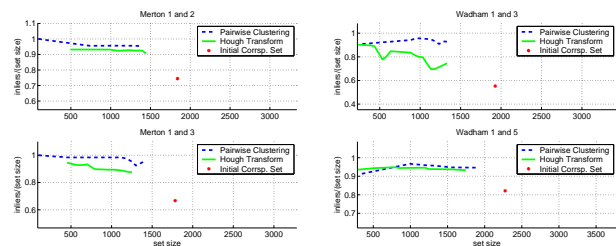
Figure 5. Proportion of inliers from the sets (of varying size) provided by each of the clustering methods.
