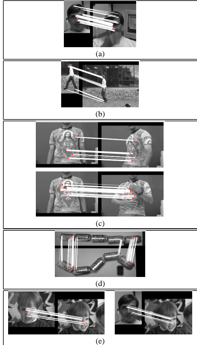
Figure 7. Recognition experiments using database of models in Fig. 6. The white lines represent the correspondences between the model found (left or top) and the test image (right or bottom) used by the verification stage. (a) Model ‘dudek’ matched despite partial occlusion, motion blur, rotation in depth, etc. (b) Articulated object ‘hedvig’ is recognized. (c) Significant non-rigid deformation and partial occlusion (right) of model ‘torso’ on the left. (d) Recognition of articulated object ‘snake of cans’. (e) Model ‘kevin’ under significant deformation. Note that we also detected a false positive (dudek) that might suggest that this method can be useful for the categorization problem.
