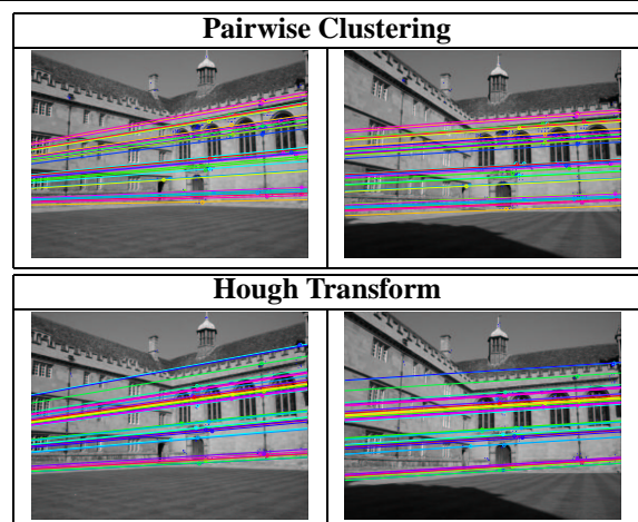
Figure 4. Epipolar lines computed from the algorithm described in [10] using the initial set of correspondences given by each clustering method (i.e., pairwise clustering and Hough).
