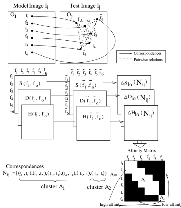
Figure 2. Grouping based on pairwise relations. Notice in the figure that correspondences 1 – 5 are semi-locally connected, while correspondence 6 is not. Therefore, we form 2 clusters, A_1 and A_2 .
